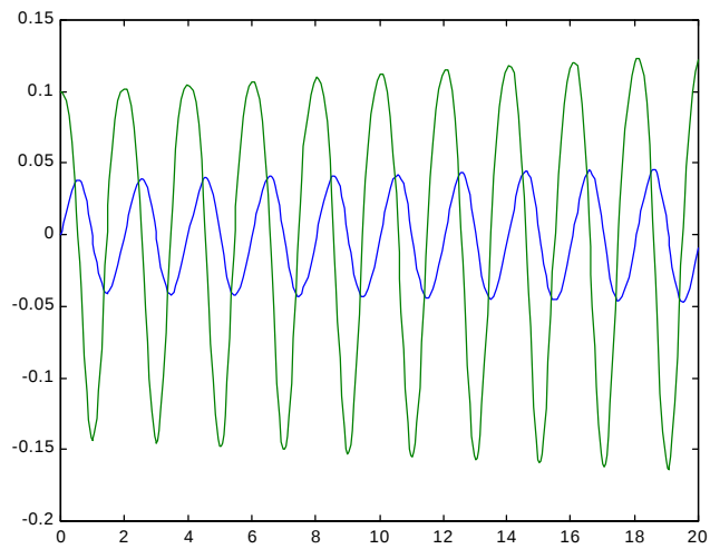
Time plot of x(1) , x(2) vs. time
